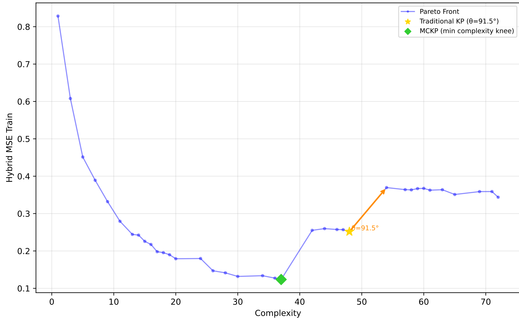
229_pwLinear - Run 5 - MVP - Hybrid MSE Train \lambda_1=0.50, \lambda_2=0.00, \lambda_3=0.00 | Difficulty: 1.00 | Method: hmr
