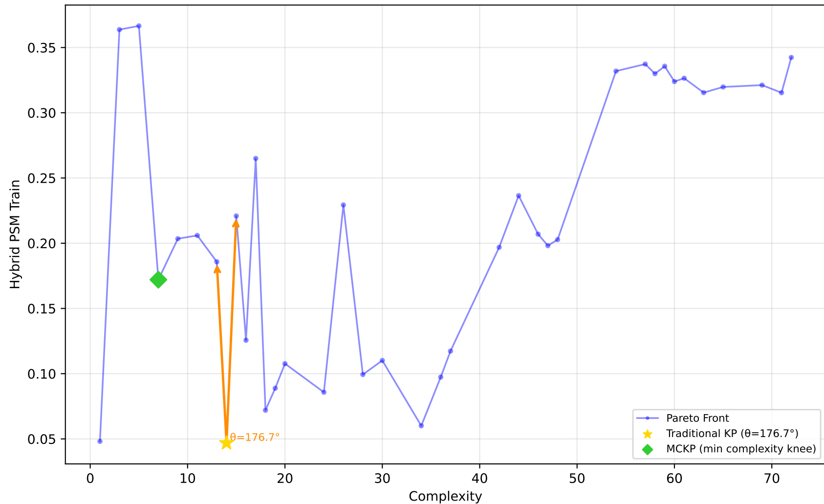
229_pwLinear - Run 5 - MVP - Hybrid PSM Train \lambda_1=0.50, \bar{\lambda}_2=0.00, \lambda_3=0.00 | Difficulty: 1.00 | Method: hmr
