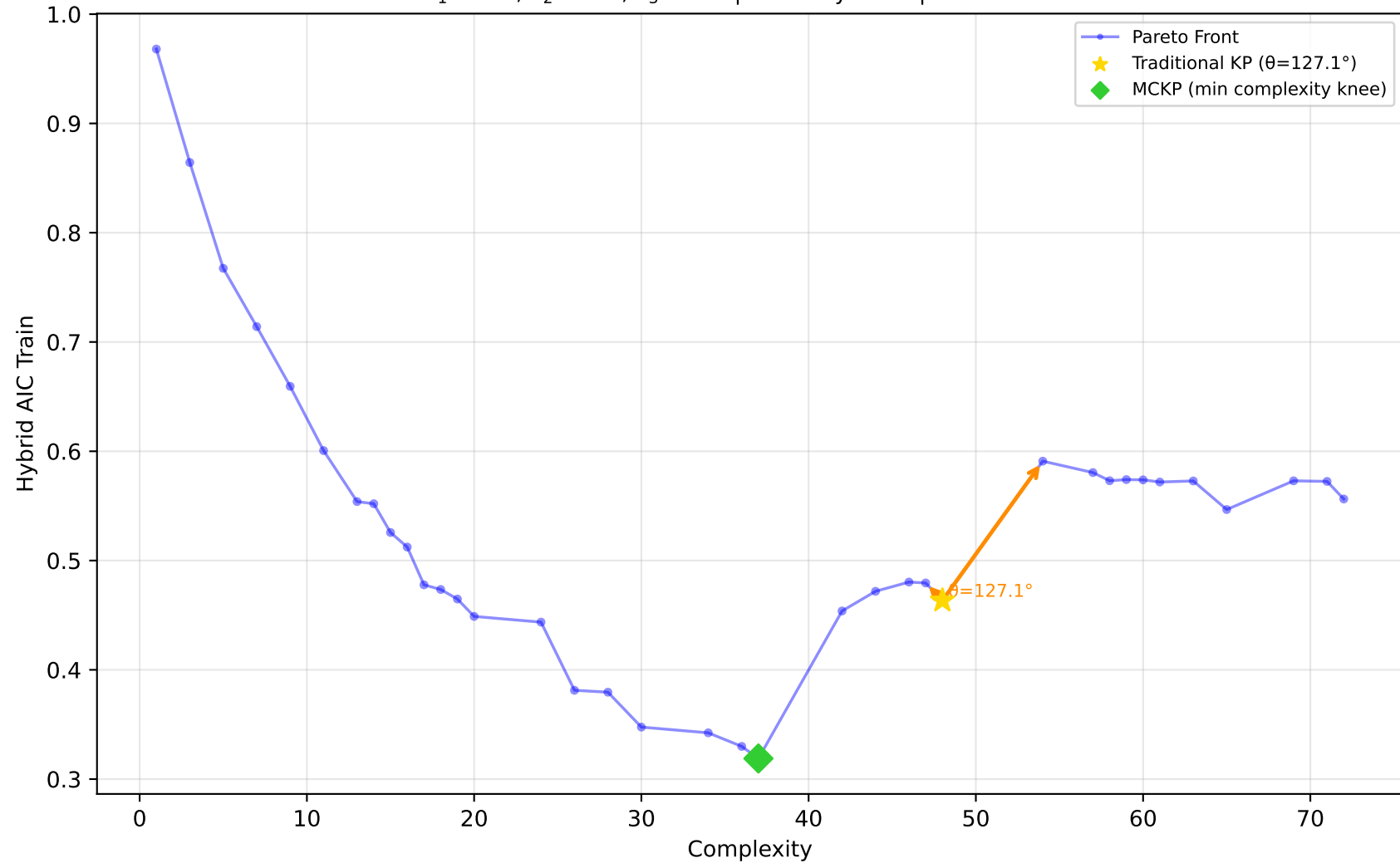
229_pwLinear - Run 5 - SVP - Hybrid AIC Train \lambda_1=0.50, \lambda_2=0.00, \lambda_3=0.00 | Difficulty: 1.00 | Method: hmr
