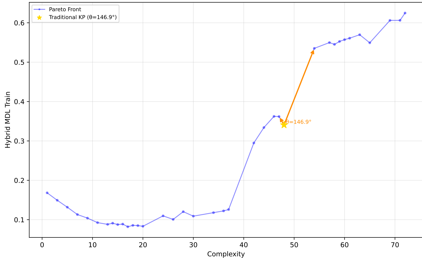
229_pwLinear - Run 5 - SVP - Hybrid MDL Train \lambda_1=0.50, \lambda_2=0.10, \lambda_3=0.00 | Difficulty: 1.00 | Method: hmr
