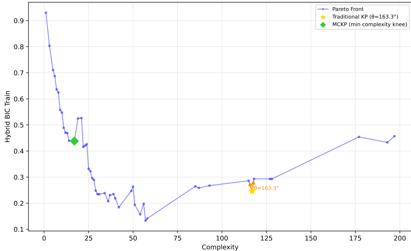
229_pwLinear - Run 6 - MVP - Hybrid BIC Train \lambda_1=0.50, \lambda_2=0.00, \lambda_3=0.00 | Difficulty: 1.00 | Method: hmr
