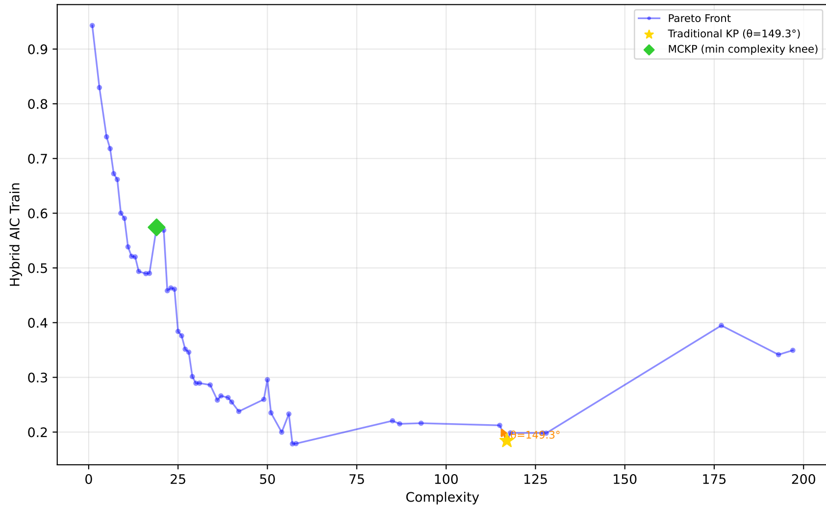
229_pwLinear - Run 6 - SVP - Hybrid AIC Train \lambda_1=0.50, \lambda_2=0.10, \lambda_3=0.00 | Difficulty: 1.00 | Method: hmr
