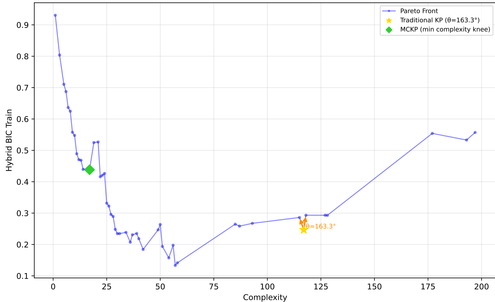
229_pwLinear - Run 6 - SVP - Hybrid BIC Train \lambda_1=0.50, \lambda_2=0.10, \lambda_3=0.00 | Difficulty: 1.00 | Method: hmr
