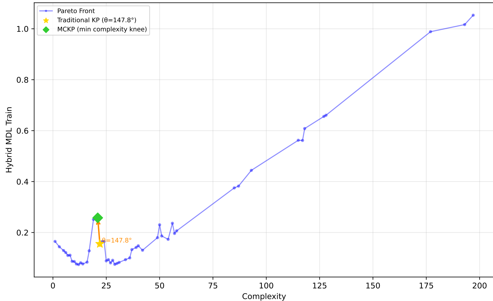
229_pwLinear - Run 6 - SVP - Hybrid MDL Train \lambda_1=0.50, \lambda_2=0.00, \lambda_3=0.00 | Difficulty: 1.00 | Method: hmr
