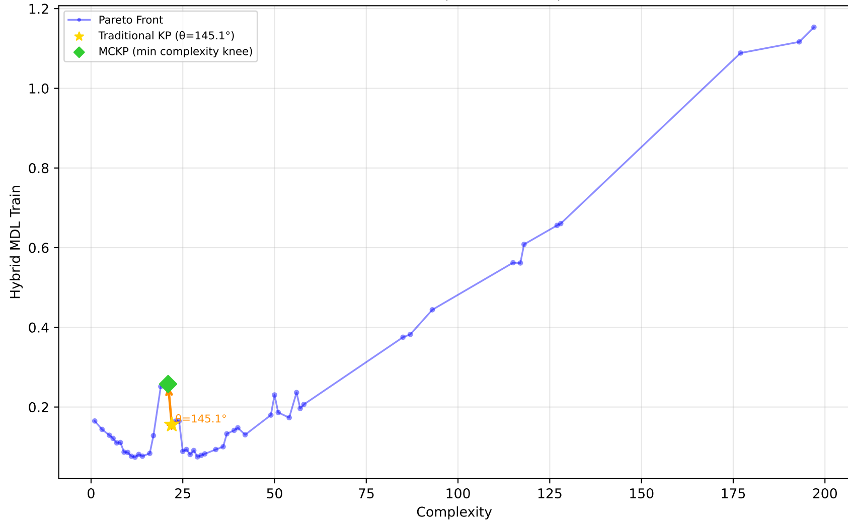
229_pwLinear - Run 6 - SVP - Hybrid MDL Train \lambda_1=0.50, \bar{\lambda}_2=0.10, \lambda_3=0.00 | Difficulty: 1.00 | Method: hmr
