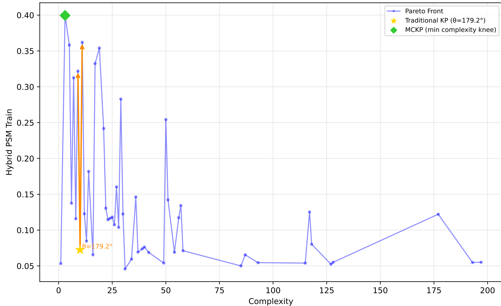
229_pwLinear - Run 6 - SVP - Hybrid PSM Train \lambda_1=0.50, \bar{\lambda}_2=0.00, \lambda_3=0.00 | Difficulty: 1.00 | Method: hmr
