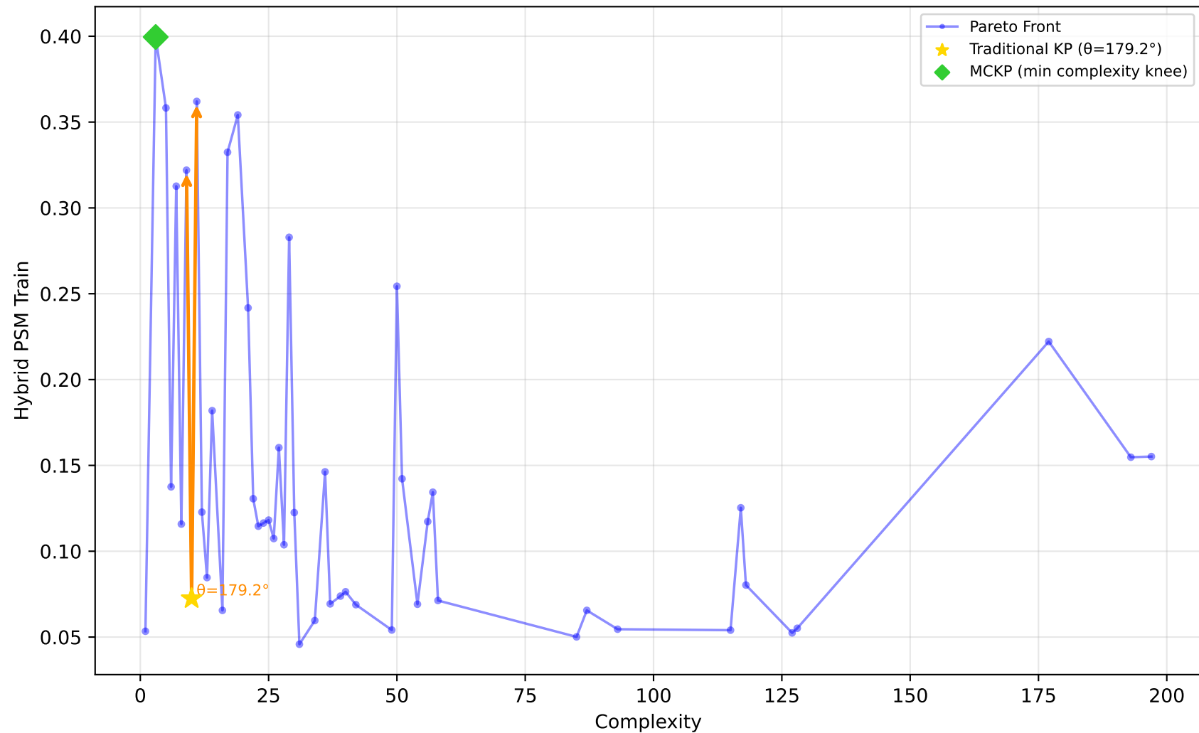
229_pwLinear - Run 6 - SVP - Hybrid PSM Train \lambda_1=0.50, \bar{\lambda}_2=0.10, \lambda_3=0.00 | Difficulty: 1.00 | Method: hmr
