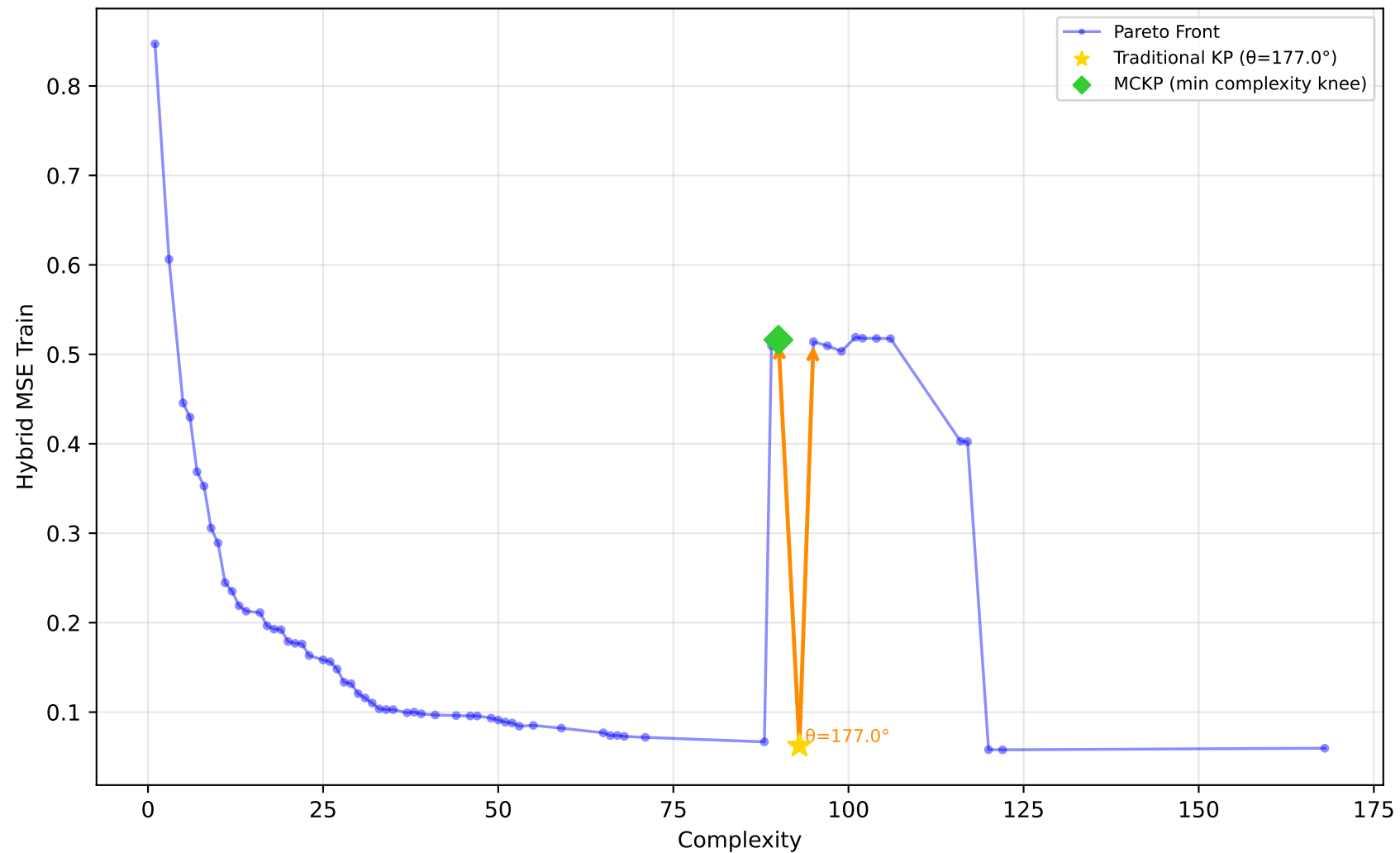
229_pwLinear - Run 7 - MVP - Hybrid MSE Train \lambda_1=0.50, \lambda_2=0.00, \lambda_3=0.00 | Difficulty: 1.00 | Method: hmr
