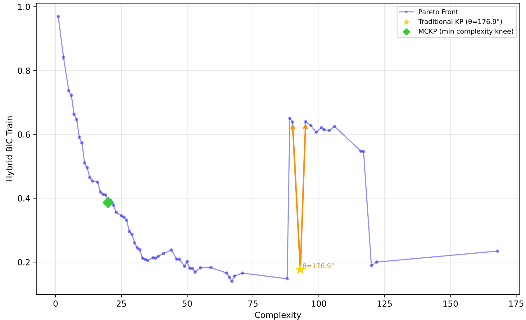
229_pwLinear - Run 7 - SVP - Hybrid BIC Train \lambda_1=0.50, \lambda_2=0.00, \lambda_3=0.00 | Difficulty: 1.00 | Method: hmr
