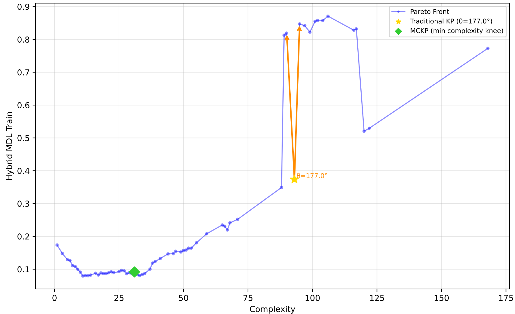
229_pwLinear - Run 7 - SVP - Hybrid MDL Train \lambda_1=0.50, \lambda_2=0.00, \lambda_3=0.00 | Difficulty: 1.00 | Method: hmr
