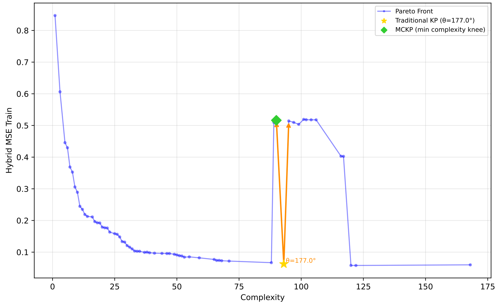
229_pwLinear - Run 7 - SVP - Hybrid MSE Train \lambda_1=0.50, \lambda_2=0.10, \lambda_3=0.00 | Difficulty: 1.00 | Method: hmr
