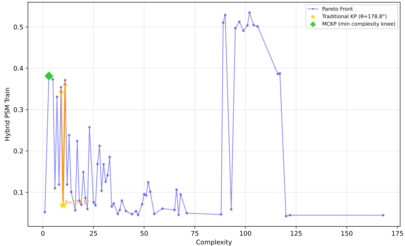
229_pwLinear - Run 7 - SVP - Hybrid PSM Train \lambda_1=0.50, \lambda_2=0.00, \lambda_3=0.00 | Difficulty: 1.00 | Method: hmr
