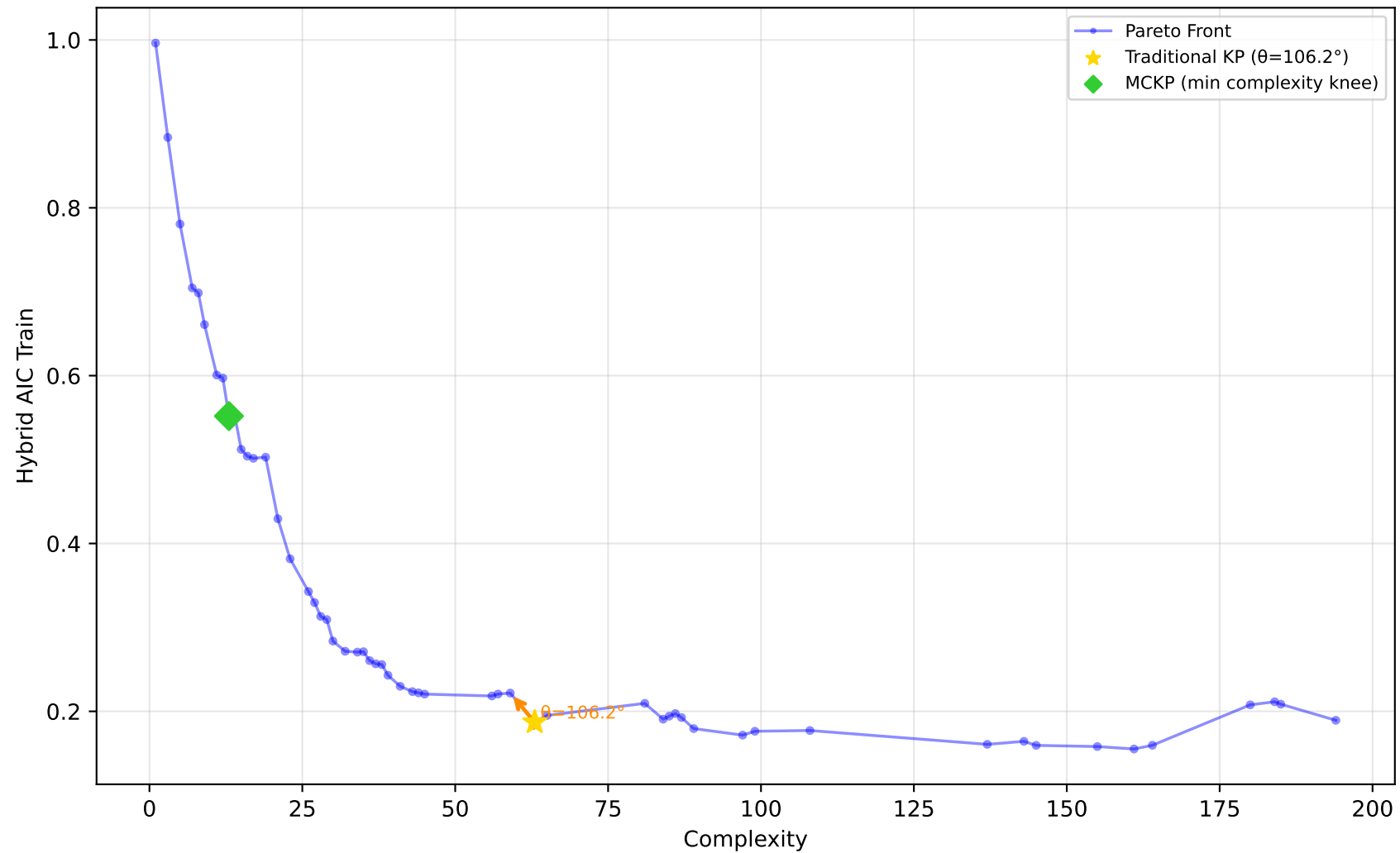
229_pwLinear - Run 8 - MVP - Hybrid AIC Train \lambda_1=0.50, \lambda_2=0.00, \lambda_3=0.00 | Difficulty: 1.00 | Method: hmr
