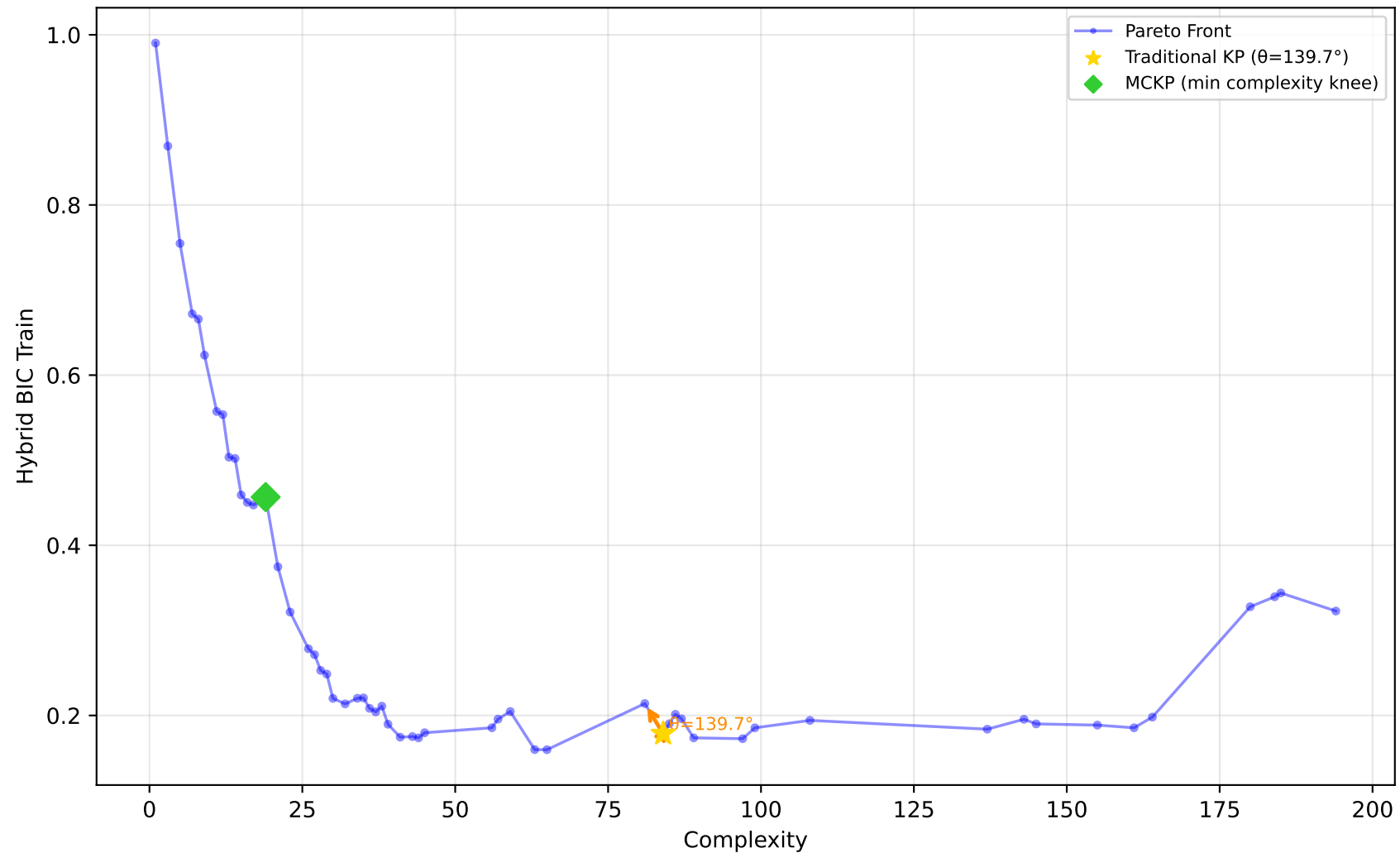
229_pwLinear - Run 8 - MVP - Hybrid BIC Train \lambda_1=0.50, \lambda_2=0.00, \lambda_3=0.00 | Difficulty: 1.00 | Method: hmr
