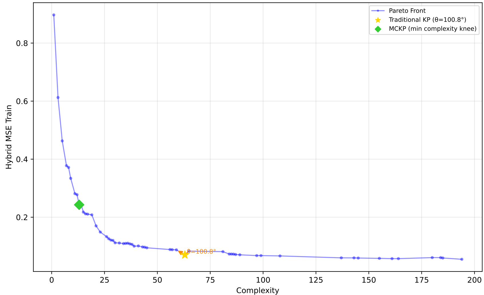
229_pwLinear - Run 8 - MVP - Hybrid MSE Train \lambda_1=0.50, \lambda_2=0.00, \lambda_3=0.00 | Difficulty: 1.00 | Method: hmr
