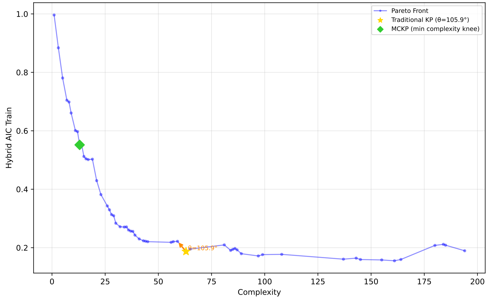
229_pwLinear - Run 8 - SVP - Hybrid AIC Train \lambda_1=0.50, \lambda_2=0.10, \lambda_3=0.00 | Difficulty: 1.00 | Method: hmr
