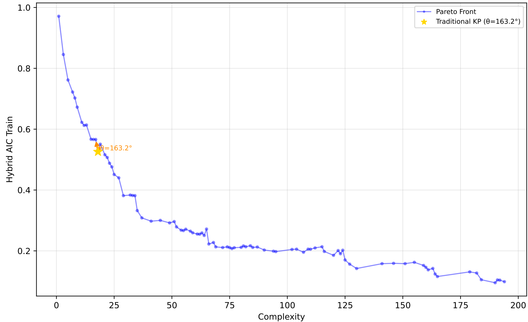
229_pwLinear - Run 9 - MVP - Hybrid AIC Train \lambda_1=0.50, \lambda_2=0.00, \lambda_3=0.00 | Difficulty: 1.00 | Method: hmr
