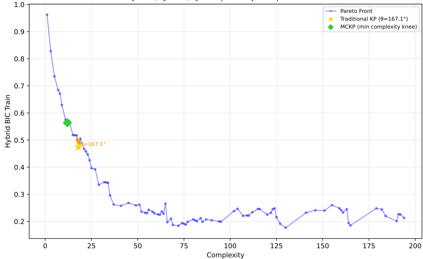
229_pwLinear - Run 9 - MVP - Hybrid BIC Train \lambda_1=0.50, \lambda_2=0.00, \lambda_3=0.00 | Difficulty: 1.00 | Method: hmr
