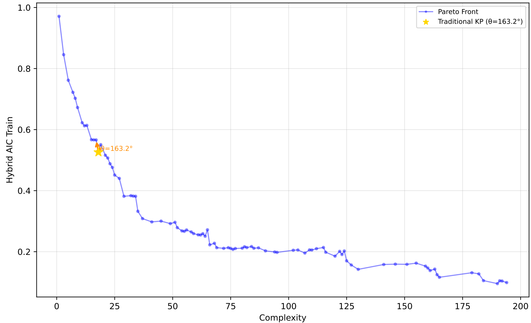
229_pwLinear - Run 9 - SVP - Hybrid AIC Train \lambda_1=0.50, \lambda_2=0.10, \lambda_3=0.00 | Difficulty: 1.00 | Method: hmr
