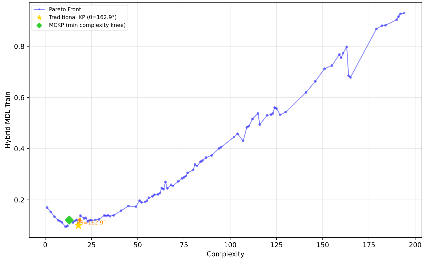
229_pwLinear - Run 9 - SVP - Hybrid MDL Train \lambda_1=0.50, \lambda_2=0.10, \lambda_3=0.00 | Difficulty: 1.00 | Method: hmr
