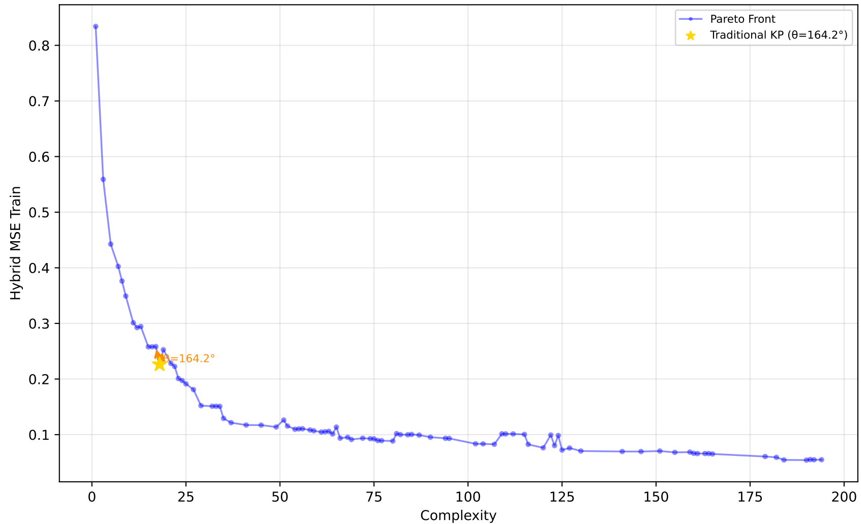
229_pwLinear - Run 9 - SVP - Hybrid MSE Train \lambda_1=0.50, \lambda_2=0.10, \lambda_3=0.00 | Difficulty: 1.00 | Method: hmr
