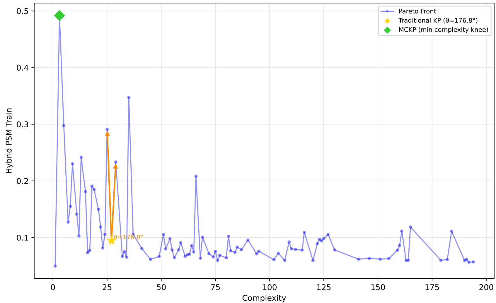
229_pwLinear - Run 9 - SVP - Hybrid PSM Train \lambda_1=0.50, \lambda_2=0.10, \lambda_3=0.00 | Difficulty: 1.00 | Method: hmr
