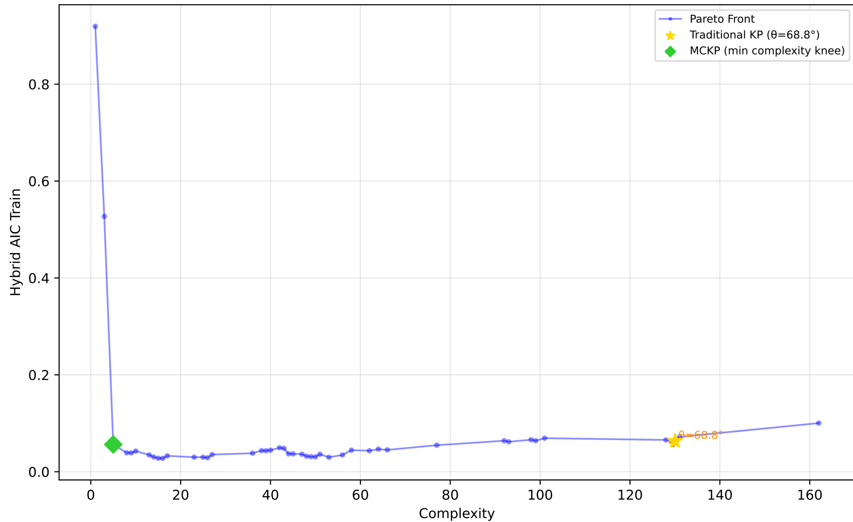
519_vinnie - Run 10 - SVP - Hybrid AIC Train \lambda_1=0.00, \lambda_2=0.00, \lambda_3=0.00 | Difficulty: 0.84 | Method: hmr
