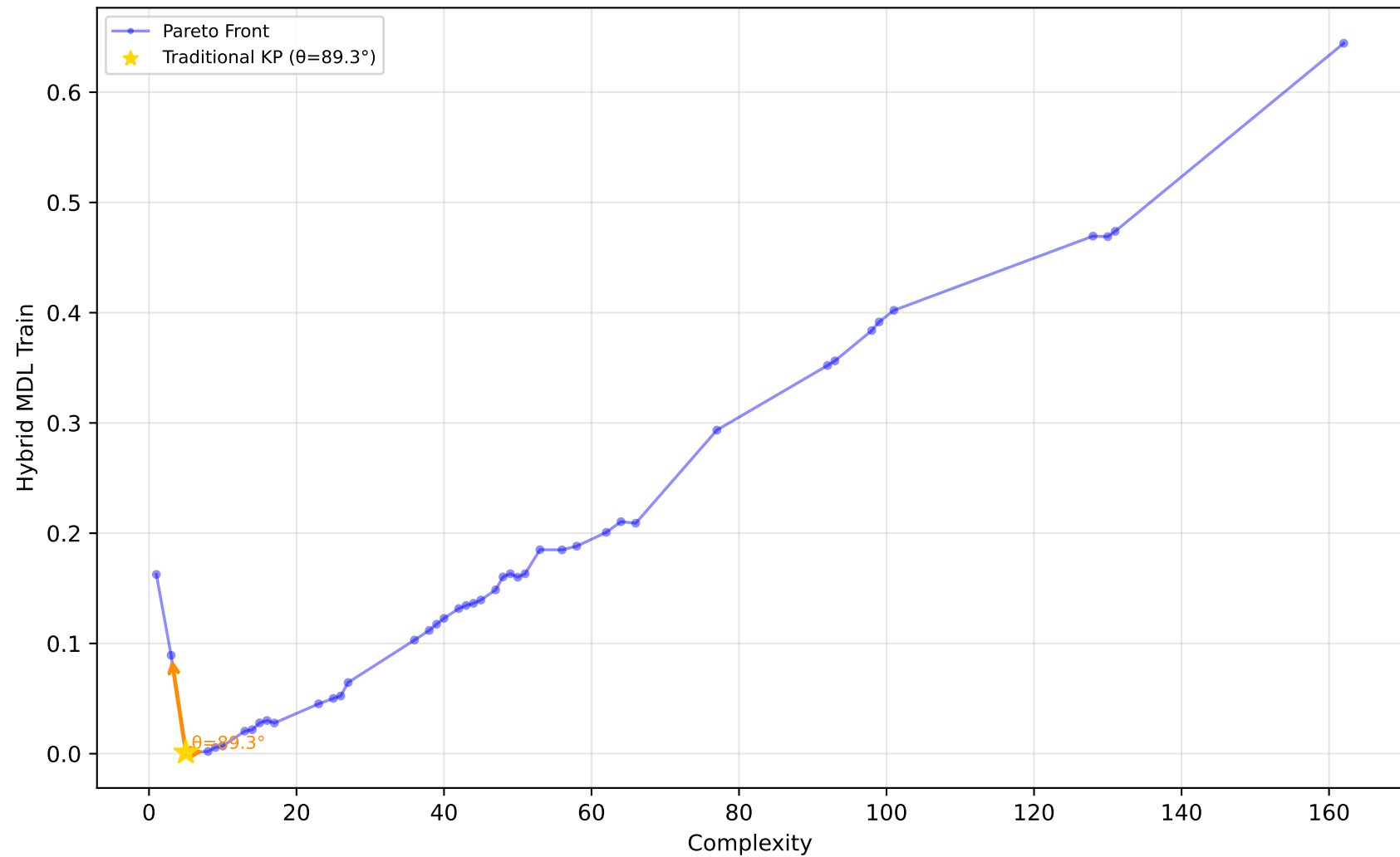
519_vinnie - Run 10 - SVP - Hybrid MDL Train \lambda_1=0.00, \lambda_2=0.00, \lambda_3=0.00 | Difficulty: 0.84 | Method: hmr
