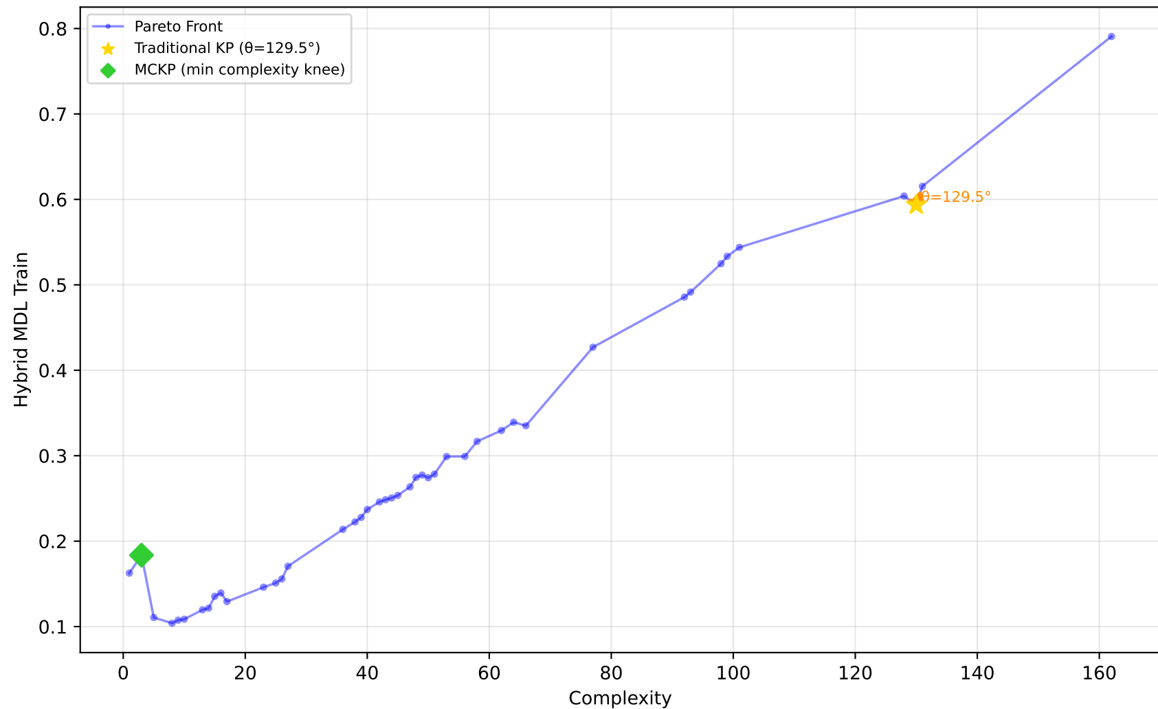
519_vinnie - Run 10 - SVP - Hybrid MDL Train \lambda_1=1.00, \lambda_2=1.00, \lambda_3=1.00 | Difficulty: 0.84 | Method: hmr
