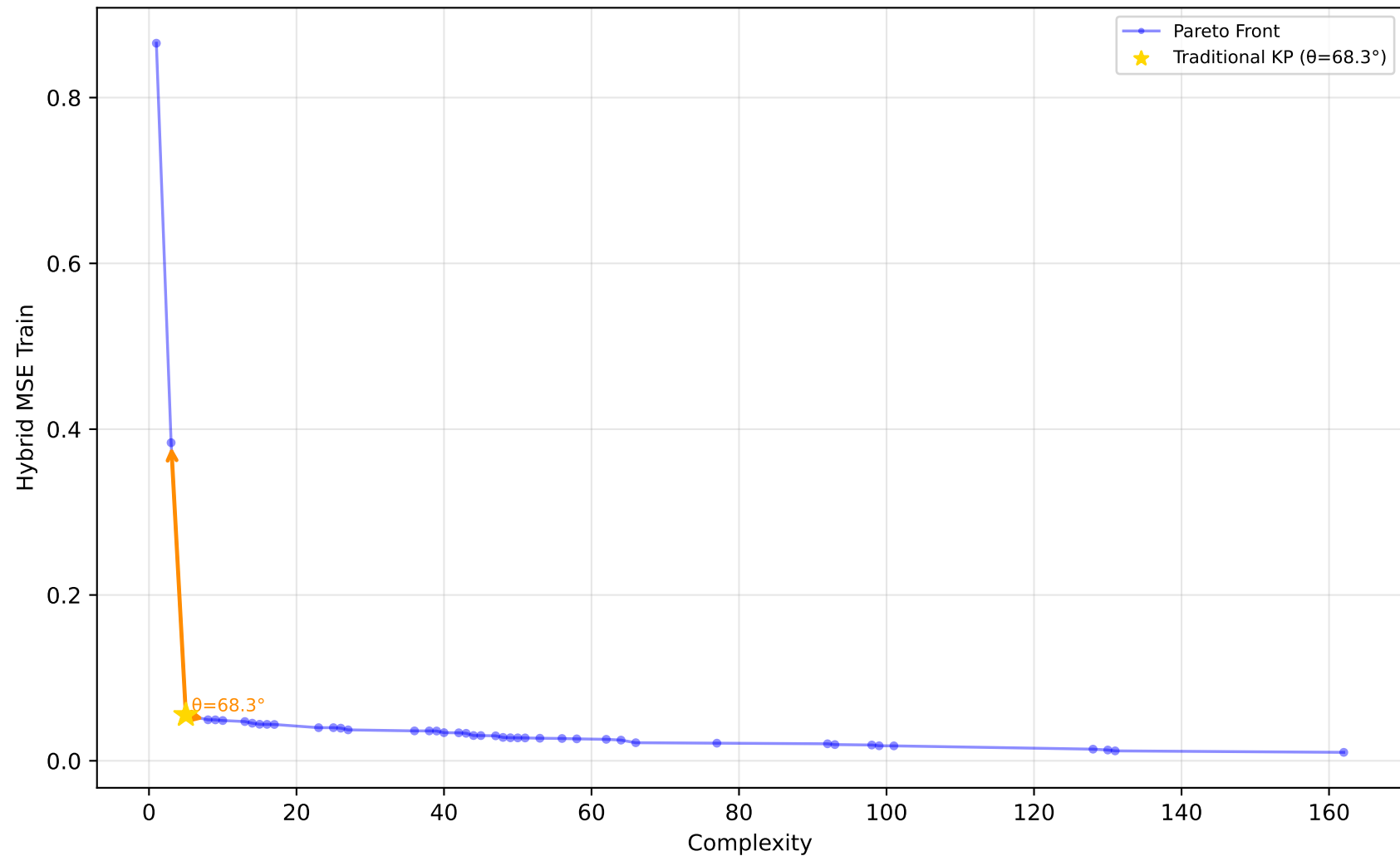
519_vinnie - Run 10 - SVP - Hybrid MSE Train \lambda_1=0.00, \lambda_2=0.00, \lambda_3=0.00 | Difficulty: 0.84 | Method: hmr
