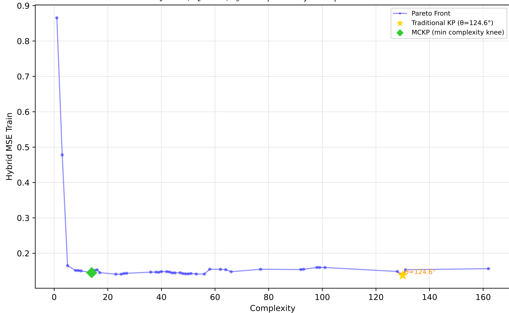
519_vinnie - Run 10 - SVP - Hybrid MSE Train \lambda_1=1.00, \lambda_2=1.00, \lambda_3=1.00 | Difficulty: 0.84 | Method: hmr
