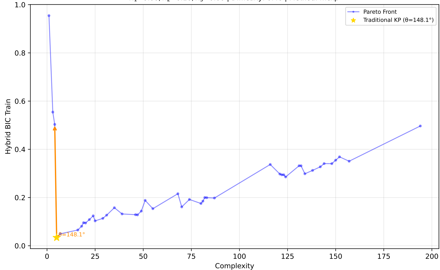
519_vinnie - Run 11 - MVP - Hybrid BIC Train \lambda_1=0.00 , \lambda_2=0.10 , \lambda_3=0.00 | Difficulty: 0.46 | Method: mckp
