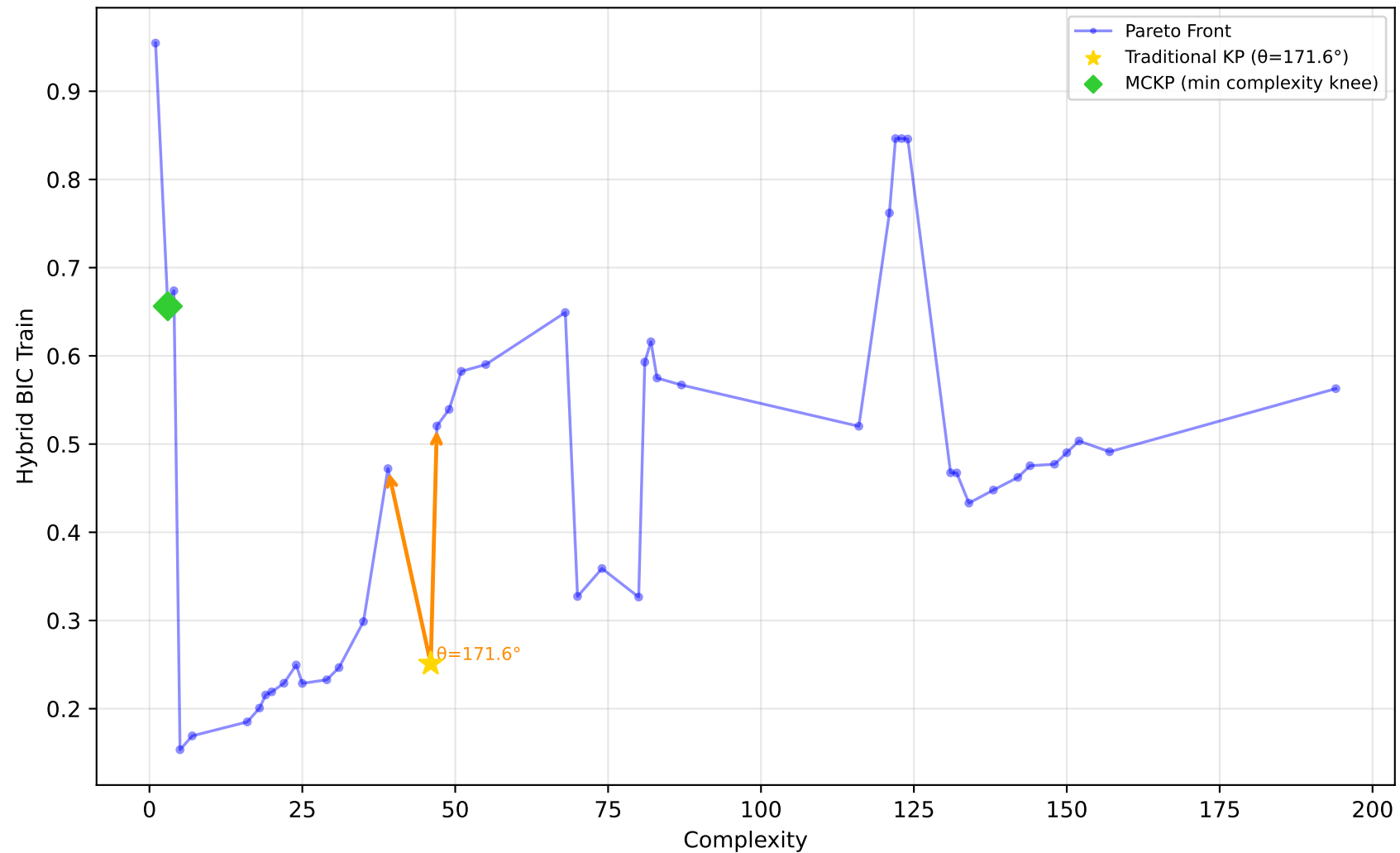
519_vinnie - Run 11 - MVP - Hybrid BIC Train \lambda_1=1.00, \lambda_2=0.00, \lambda_3=1.00 | Difficulty: 0.46 | Method: mckp
