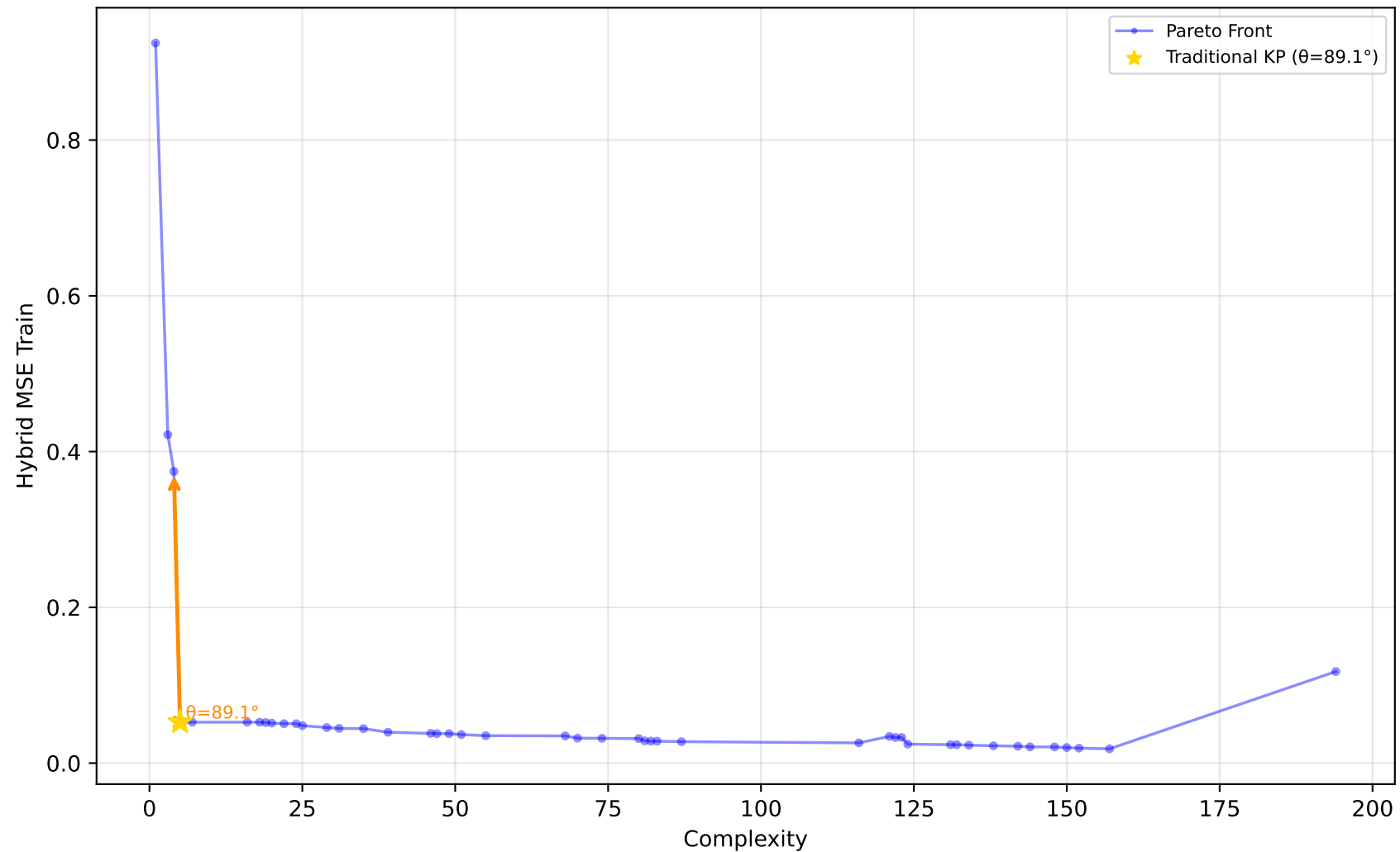
519_vinnie - Run 11 - MVP - Hybrid MSE Train \lambda_1=0.00, \lambda_2=0.10, \lambda_3=0.00 | Difficulty: 0.46 | Method: mckp
