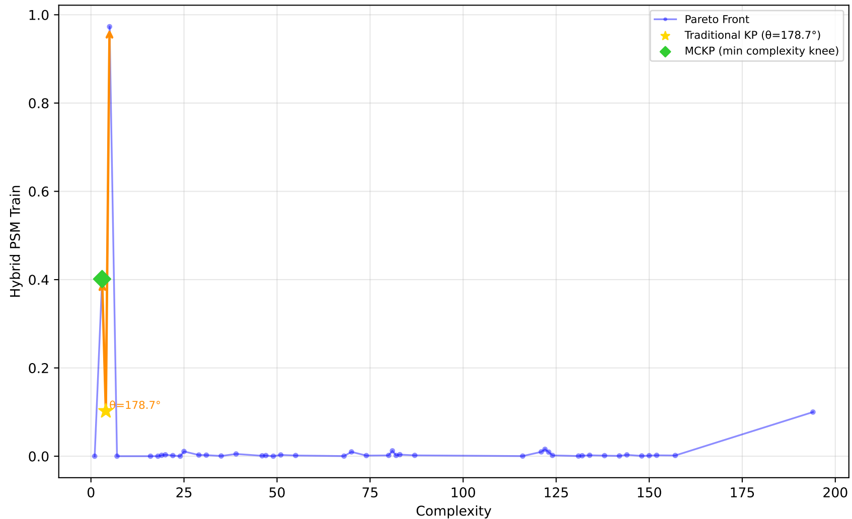
519_vinnie - Run 11 - MVP - Hybrid PSM Train \lambda_1=0.00, \lambda_2=0.10, \lambda_3=0.00 | Difficulty: 0.46 | Method: mckp
