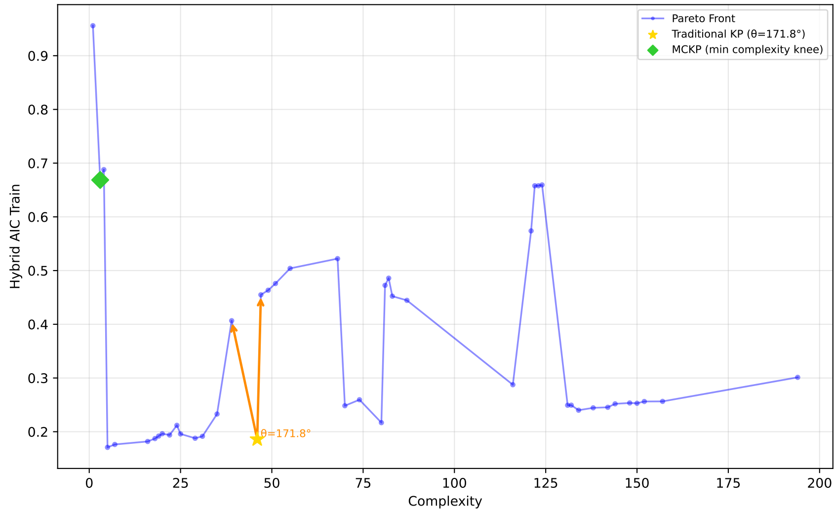
519_vinnie - Run 11 - SVP - Hybrid AIC Train \lambda_1=1.00, \lambda_2=1.00, \lambda_3=1.00 | Difficulty: 0.46 | Method: mckp
