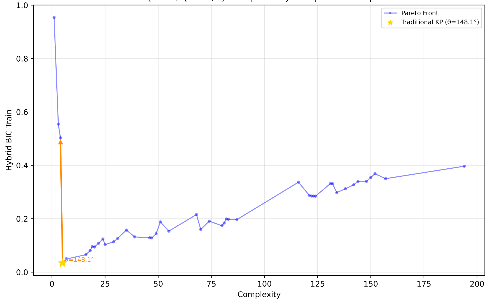
519_vinnie - Run 11 - SVP - Hybrid BIC Train \lambda_1=0.00, \lambda_2=0.00, \lambda_3=0.00 | Difficulty: 0.46 | Method: mckp
