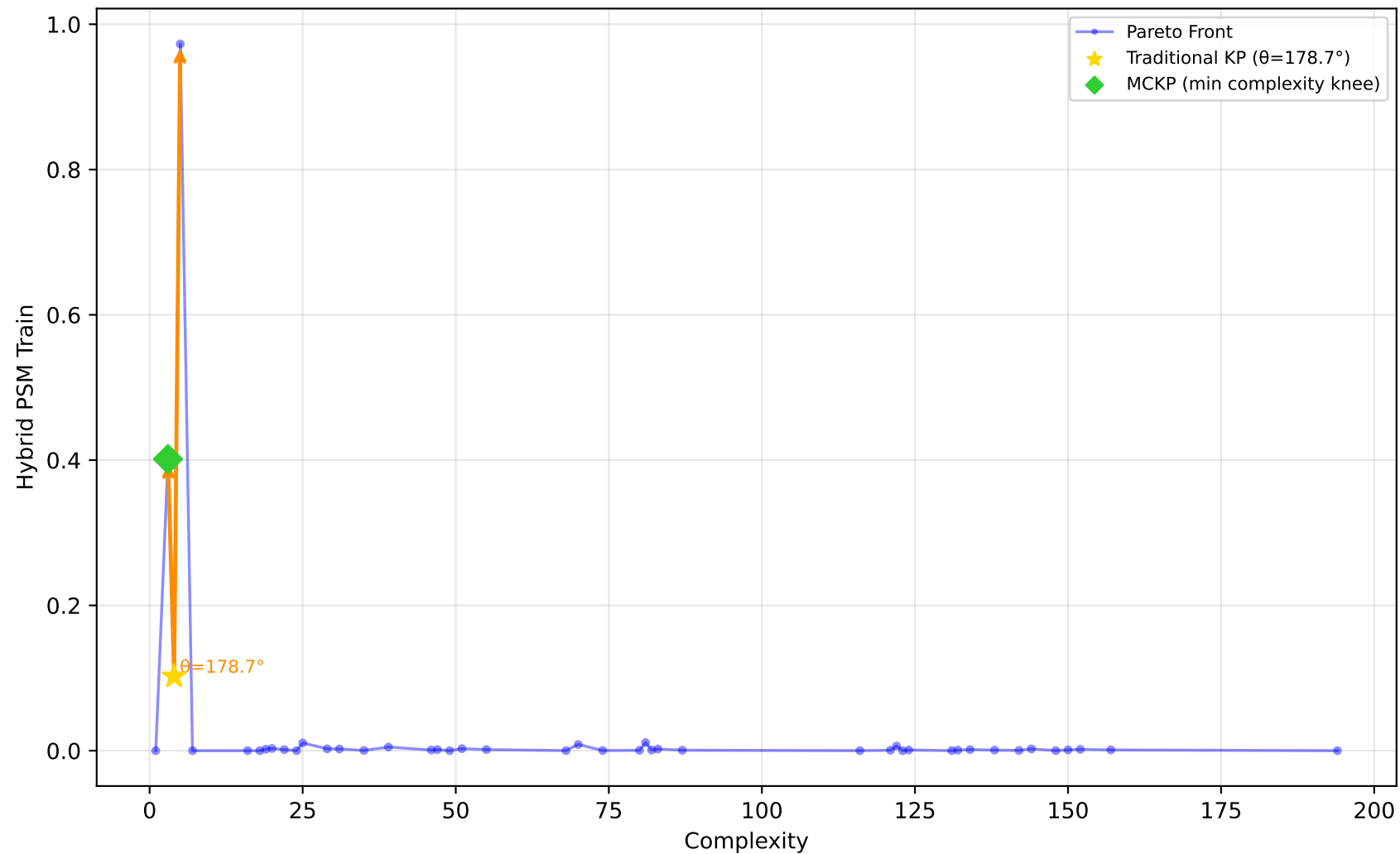
519_vinnie - Run 11 - SVP - Hybrid PSM Train \lambda_1=0.00, \lambda_2=0.00, \lambda_3=0.00 | Difficulty: 0.46 | Method: mckp
