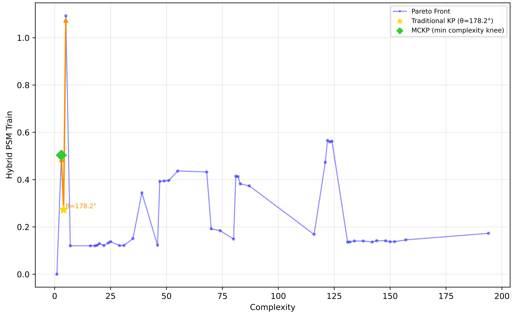
519_vinnie - Run 11 - SVP - Hybrid PSM Train \lambda_1=1.00, \lambda_2=1.00, \lambda_3=1.00 | Difficulty: 0.46 | Method: mckp
