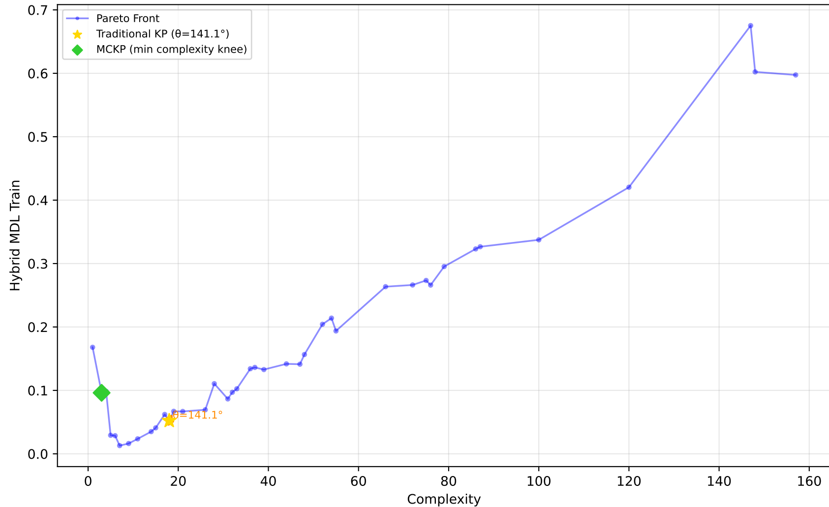
519_vinnie - Run 12 - MVP - Hybrid MDL Train \lambda_1=0.00, \lambda_2=0.10, \lambda_3=0.00 | Difficulty: 0.78 | Method: hmr
