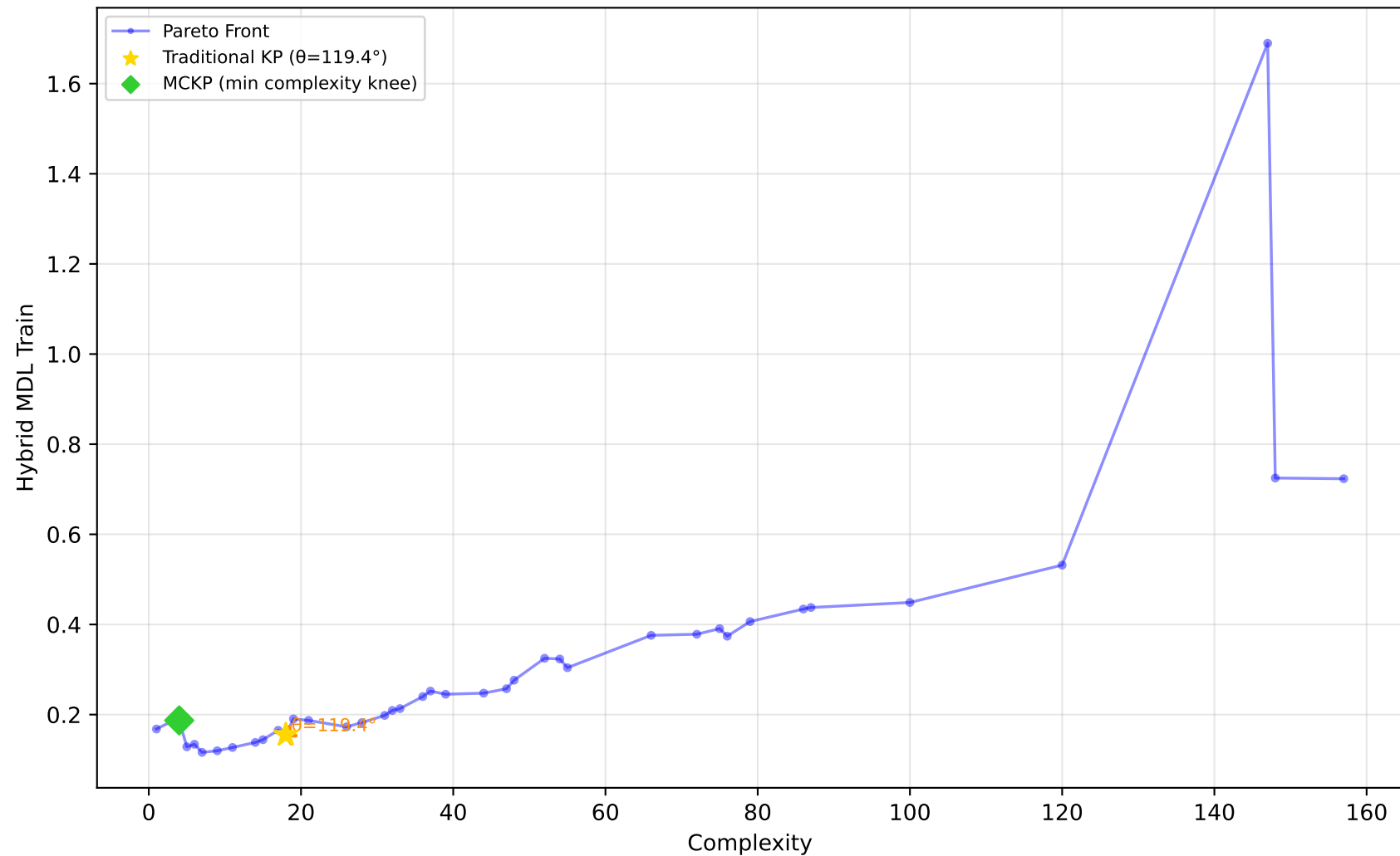
519_vinnie - Run 12 - MVP - Hybrid MDL Train \lambda_1=1.00, \lambda_2=0.00, \lambda_3=1.00 | Difficulty: 0.78 | Method: hmr
