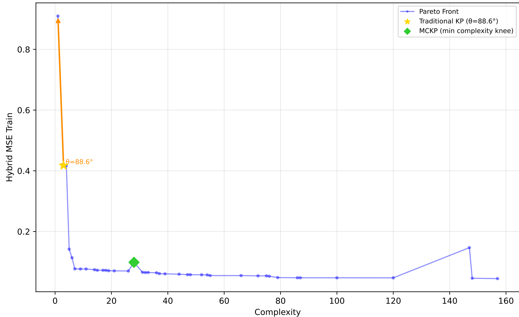
519_vinnie - Run 12 - MVP - Hybrid MSE Train \lambda_1=0.00, \lambda_2=0.10, \lambda_3=0.00 | Difficulty: 0.78 | Method: hmr
