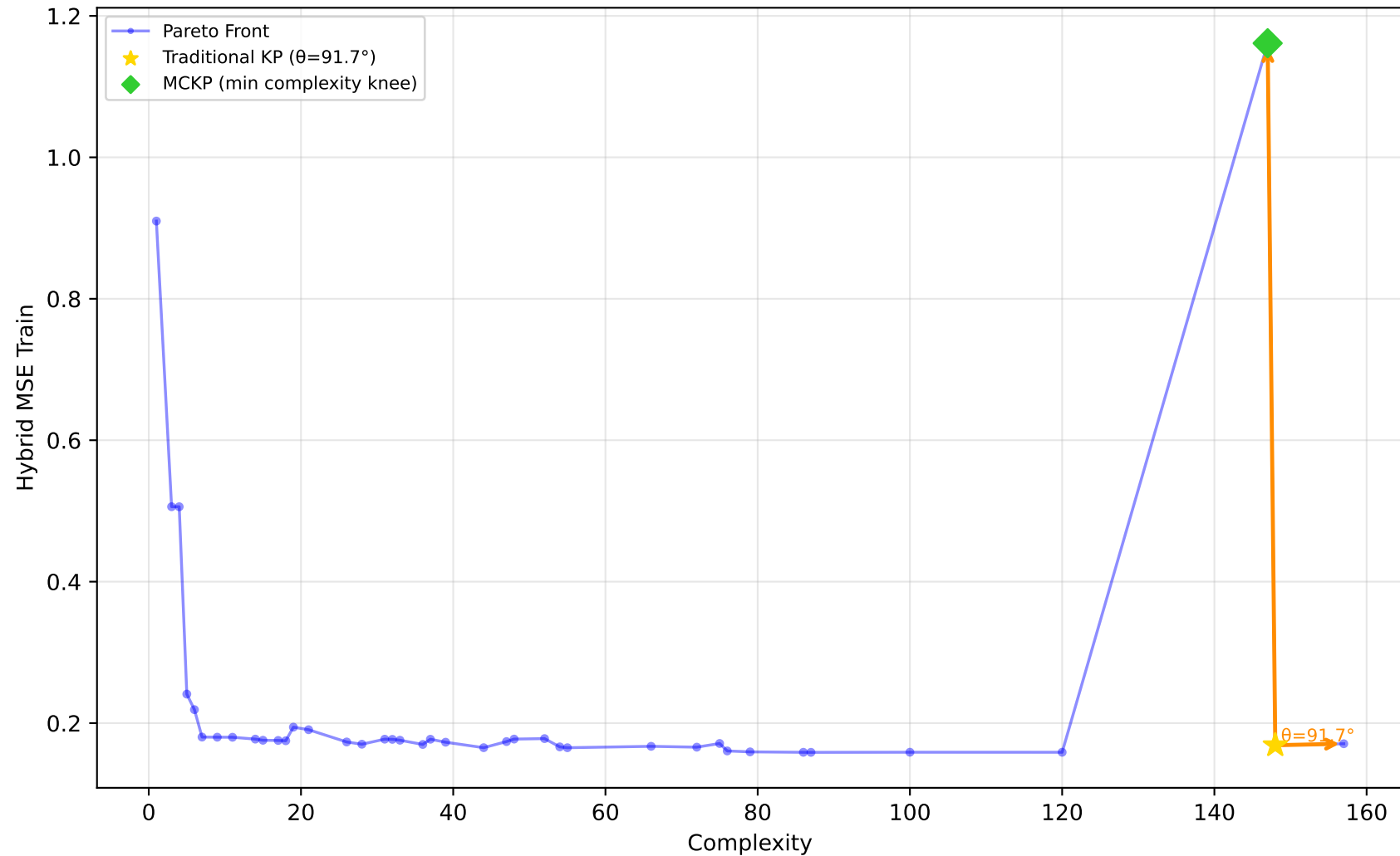
519_vinnie - Run 12 - MVP - Hybrid MSE Train \lambda_1=1.00, \lambda_2=0.00, \lambda_3=1.00 | Difficulty: 0.78 | Method: hmr
