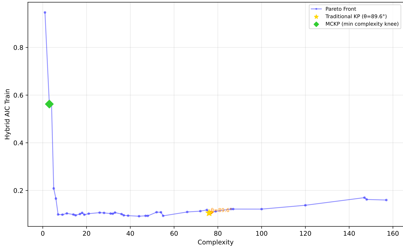
519_vinnie - Run 12 - SVP - Hybrid AIC Train \lambda_1=0.00, \lambda_2=0.00, \lambda_3=0.00 | Difficulty: 0.78 | Method: hmr
