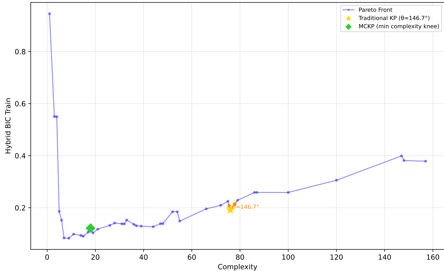
519_vinnie - Run 12 - SVP - Hybrid BIC Train \lambda_1=0.00, \lambda_2=0.00, \lambda_3=0.00 | Difficulty: 0.78 | Method: hmr
