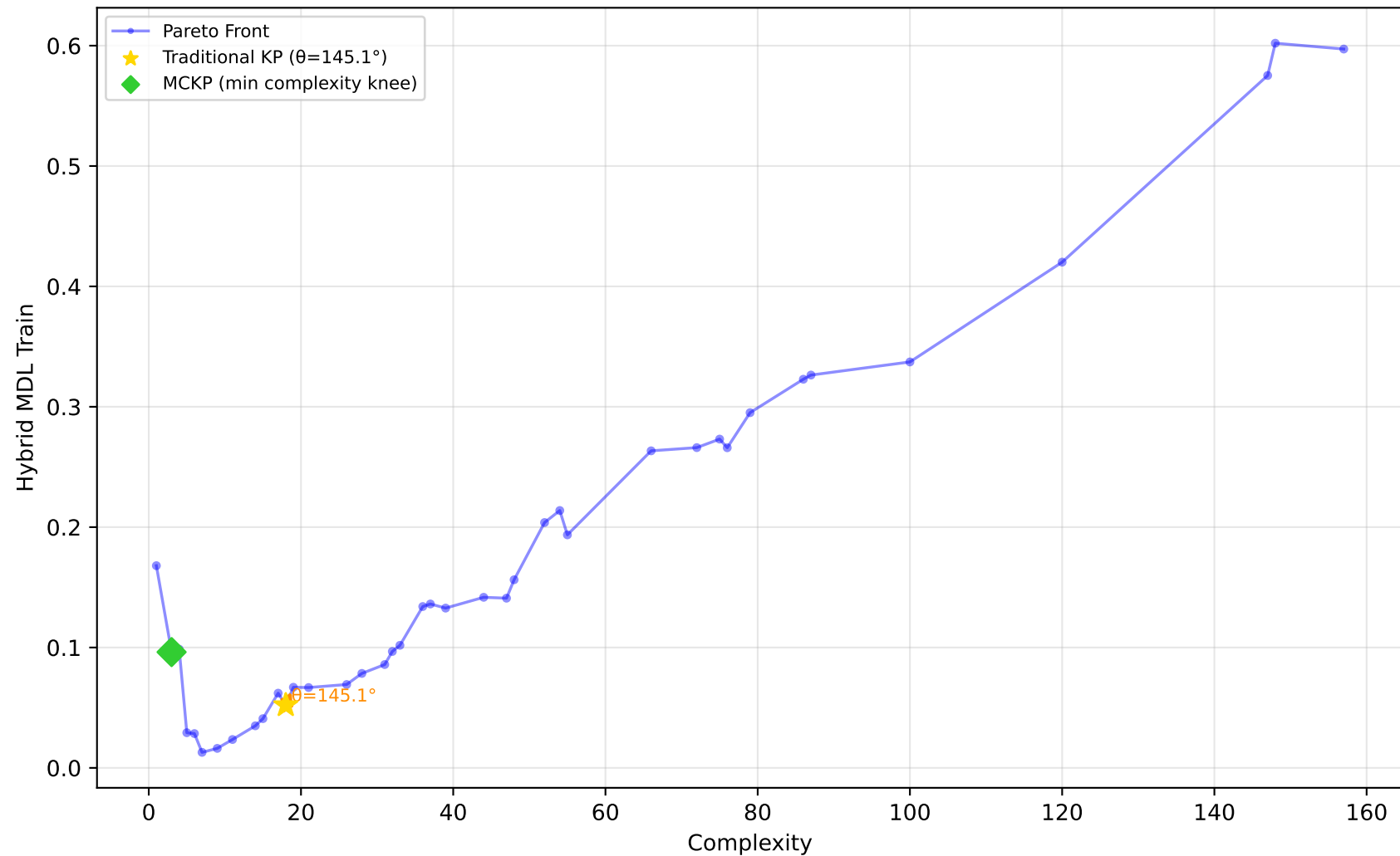
519_vinnie - Run 12 - SVP - Hybrid MDL Train \lambda_1=0.00, \lambda_2=0.00, \lambda_3=0.00 | Difficulty: 0.78 | Method: hmr
