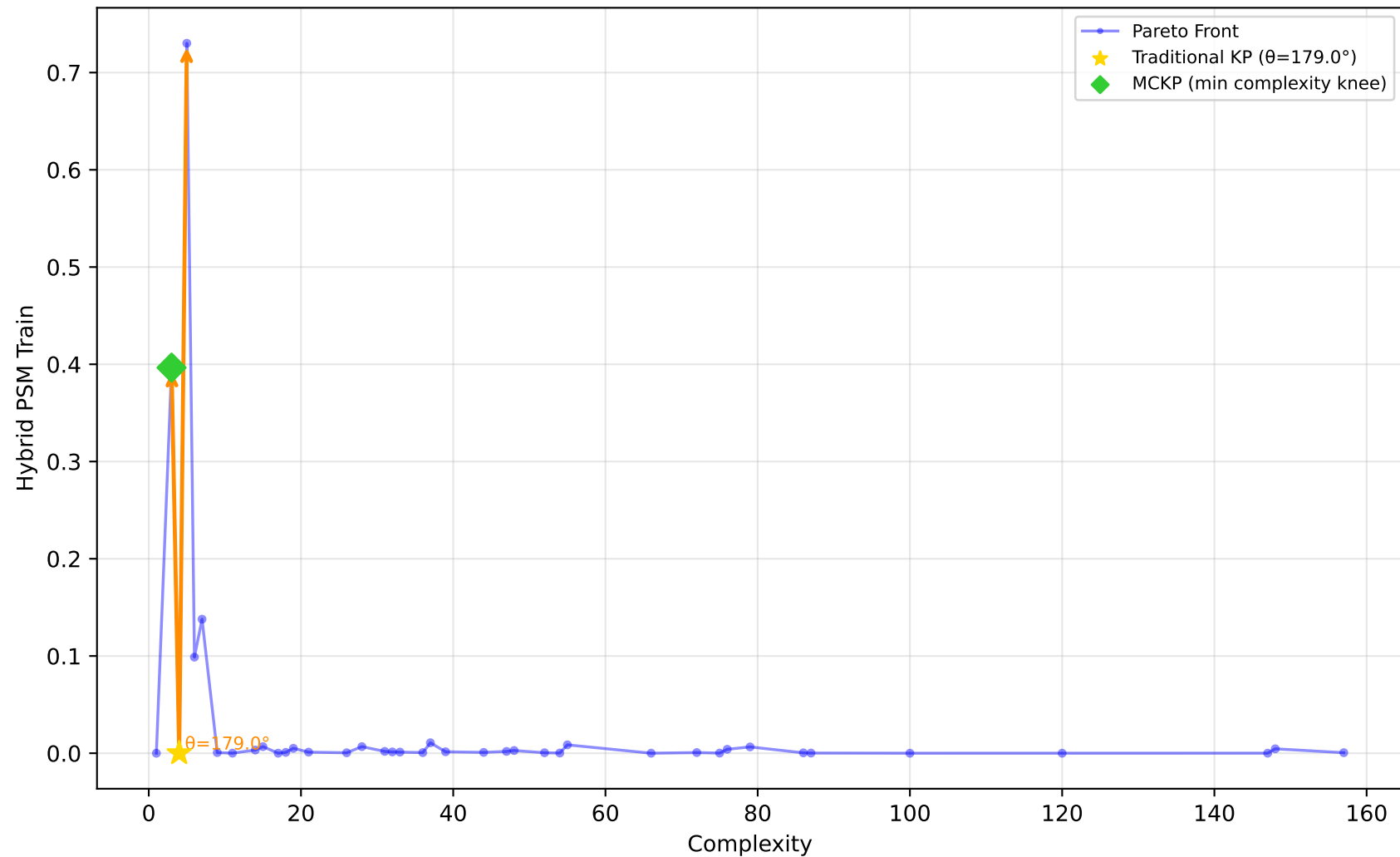
519_vinnie - Run 12 - SVP - Hybrid PSM Train \lambda_1=0.00, \lambda_2=0.00, \lambda_3=0.00 | Difficulty: 0.78 | Method: hmr
