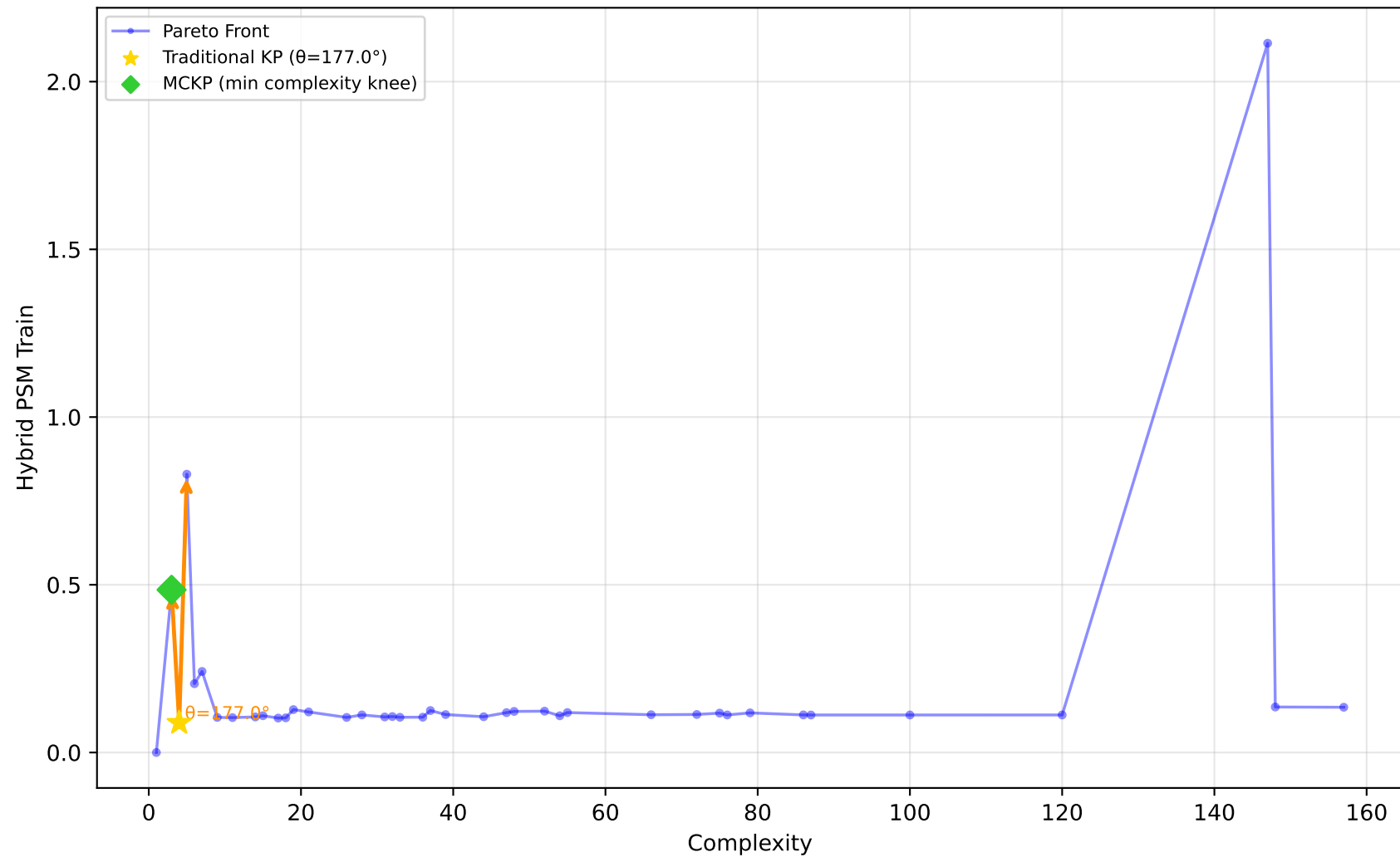
519_vinnie - Run 12 - SVP - Hybrid PSM Train \lambda_1=1.00, \lambda_2=1.00, \lambda_3=1.00 | Difficulty: 0.78 | Method: hmr
