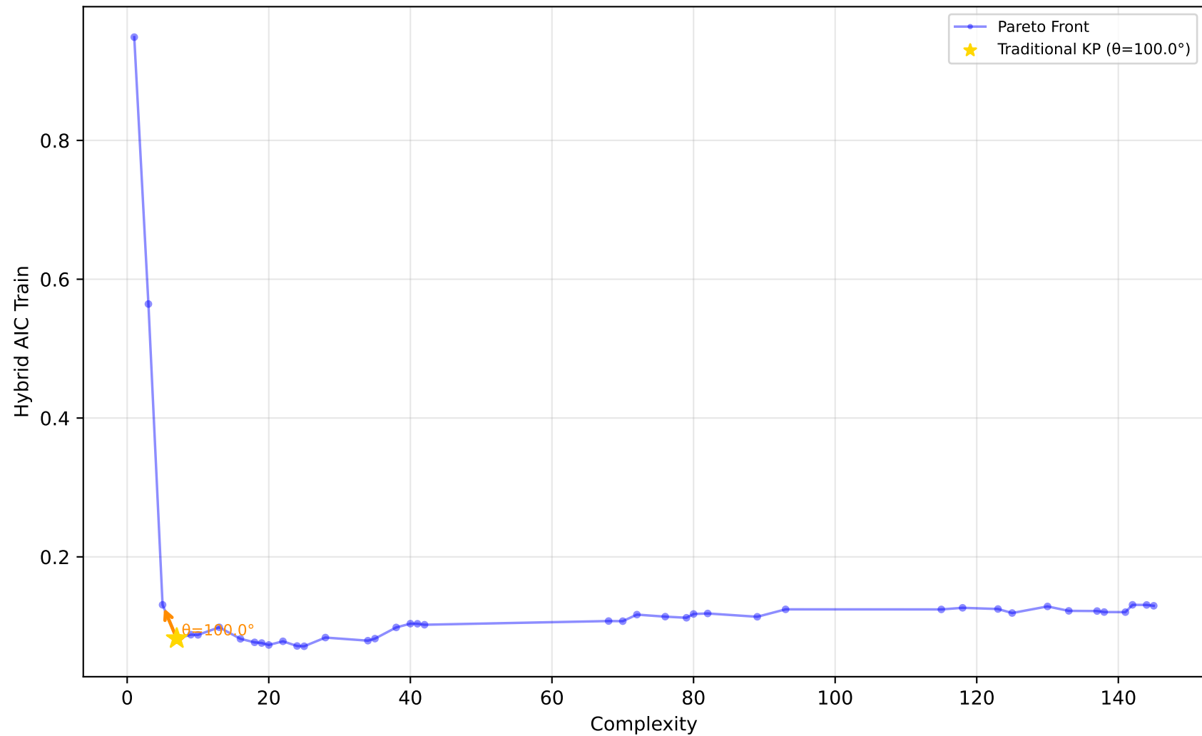
519_vinnie - Run 13 - MVP - Hybrid AIC Train \lambda_1=0.00, \lambda_2=0.10, \lambda_3=0.00 | Difficulty: 0.54 | Method: mckp
