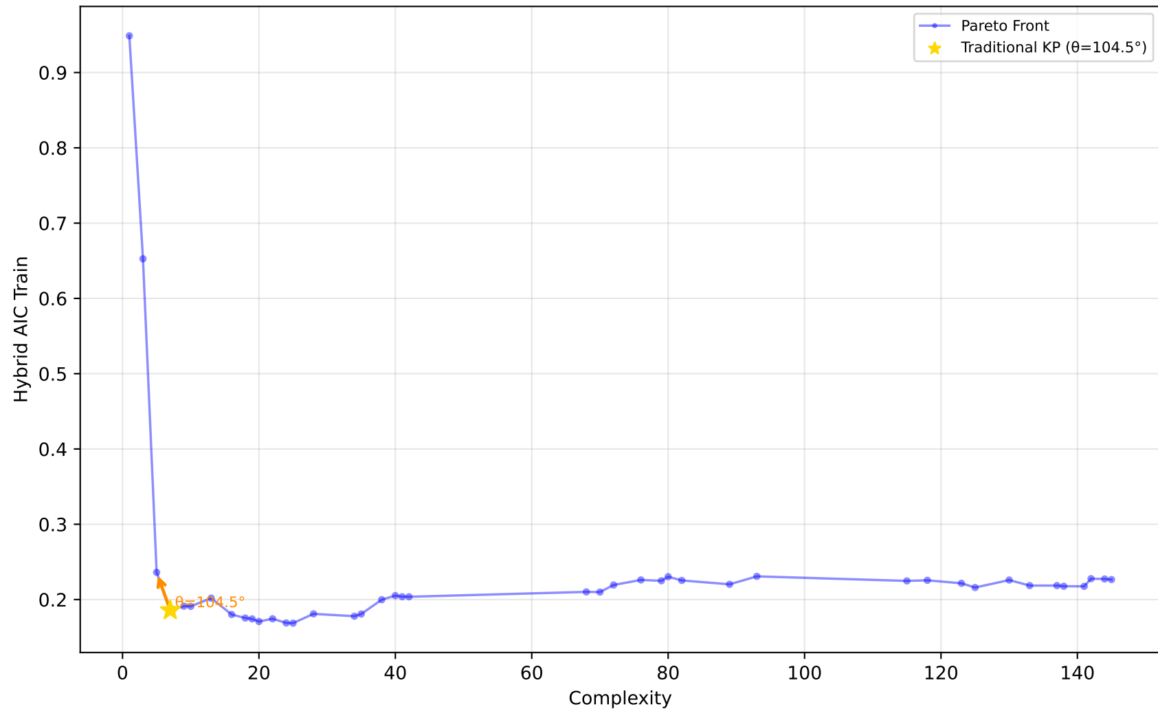
519_vinnie - Run 13 - MVP - Hybrid AIC Train \lambda_1=1.00, \lambda_2=0.00, \lambda_3=1.00 | Difficulty: 0.54 | Method: mckp
